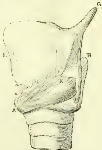
External and Sectional views of the Larynx.
